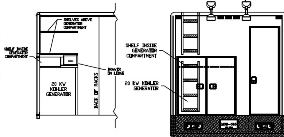
REAR-WALL ELEVATION
