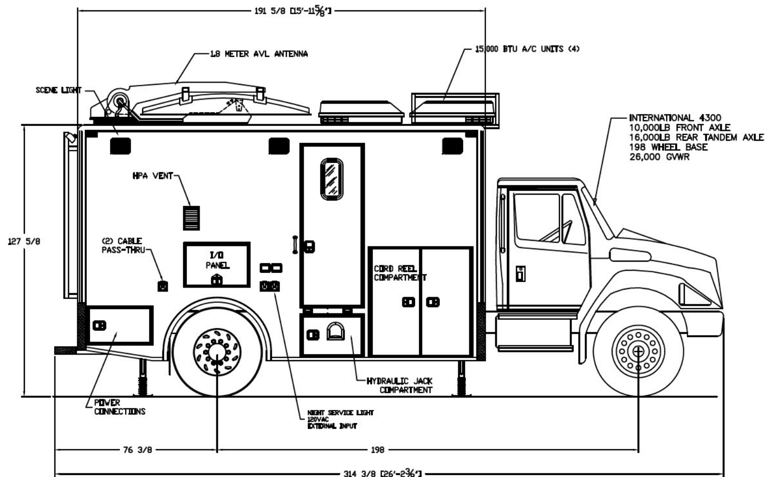
CURB-SIDE ELEVATION
