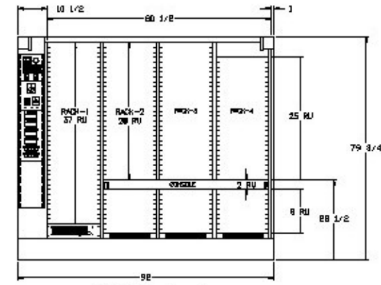
VIEW A-A RACKS 1 THROUGH 4
