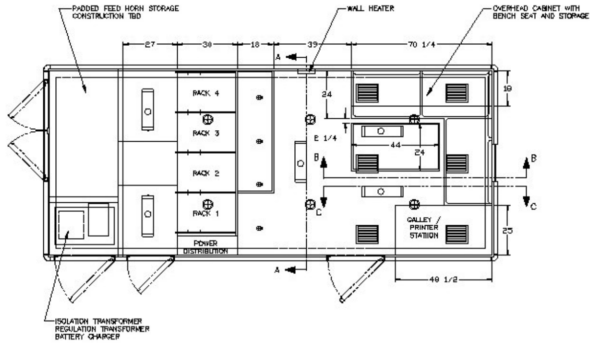
FLOOR PLAN
